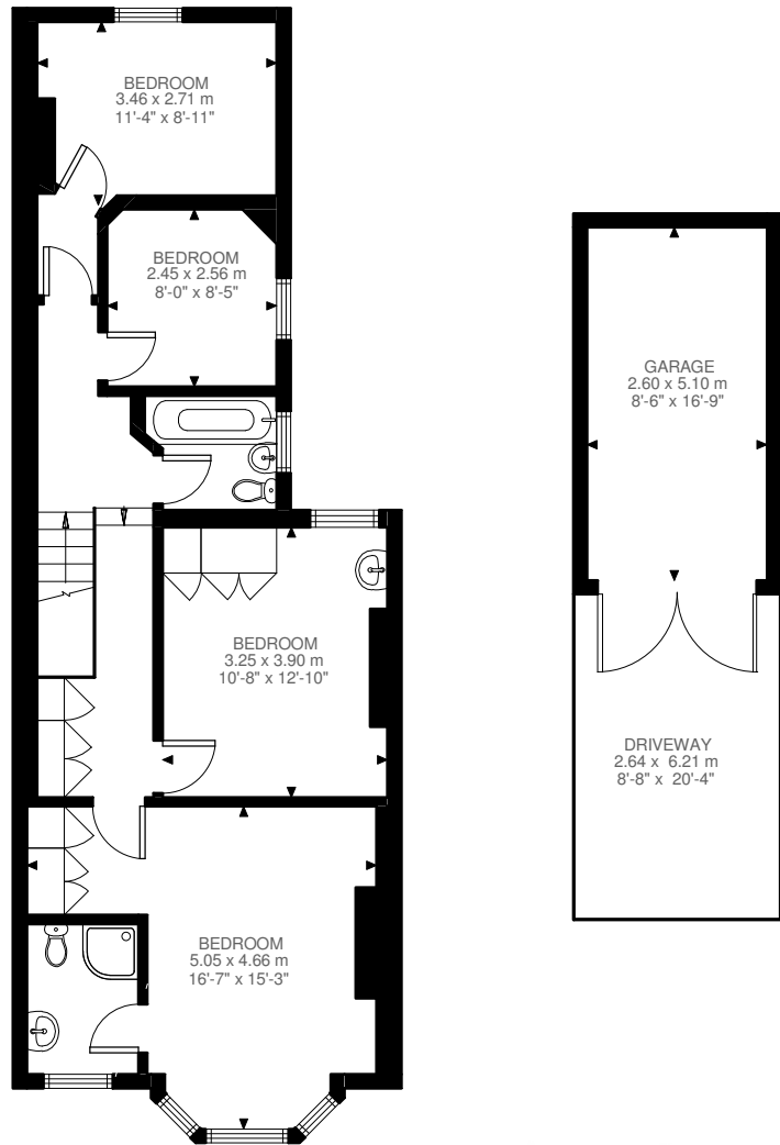
First Floor
